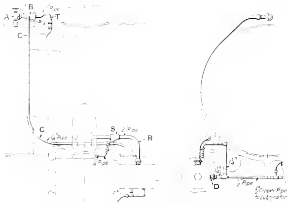
Arrangement of Piping, Vincent Drifting Valve
